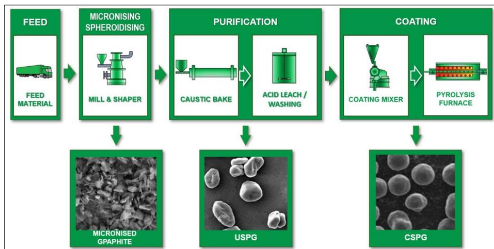
Above: Simplified Flow sheet for the Proposed Collie Graphite BAM Facility
